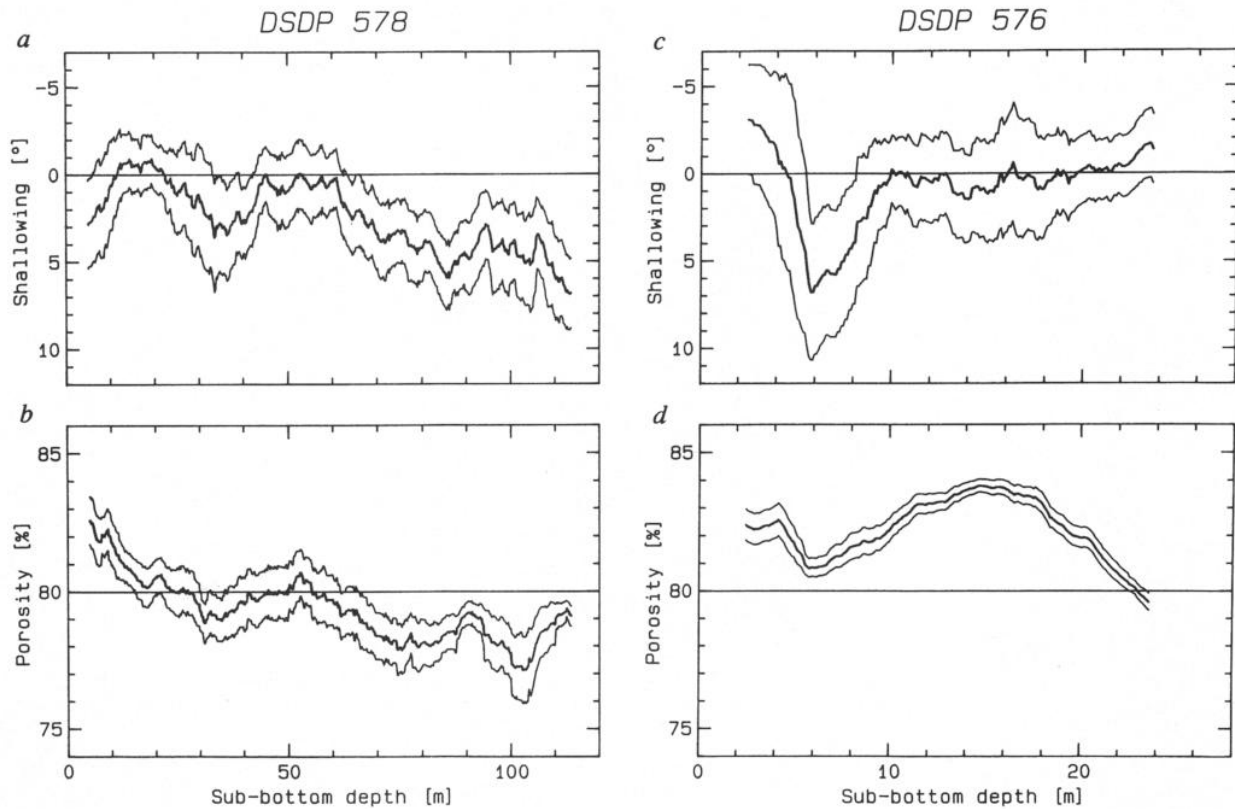
Fig. 7. A running average of the inclination and porosity data in depth domains. The shallowing was calculated with the same method as in Figure 5, with a fixed depth interval running window. The running averages are shown by a bold curve, enveloped by 95% confidence limits. (a) Average inclination shallowing at site 578. (b) Average porosities at site 578. The site 578 data were calculated every 0.2 m using a 10-m running window between 5.0 and 113.6 m (544 values). (c) Average inclination shallowing at site 576. (d) Average porosities at site 576. The site 576 averages were calculated every 0.1 m using a 5-m running window centered between 2.5 and 23.6 m (212 values). The downhole trends are now more visible than in Figures 4 and 6.
