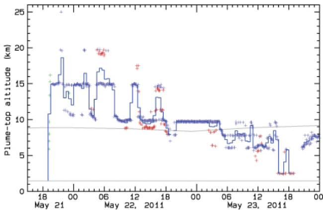
Figure 5. The time series of the 5-min detected plume-top altitude (km a.s.l.) during the first 53 h of the eruption. Altitude estimates are from the C-band weather radar (blue) and the X-band mobile radar (red), as well as the initial rise of the plume estimated from photographs (green). The altitude of the tropopause, observed by Keflavík radiosondes is shown at about 9 km a.s.l. (gray). The lower gray line represents the altitude of the Grímsvötn caldera. A 30-min average plume-top altitude of all the estimates is shown by the blue curve.
