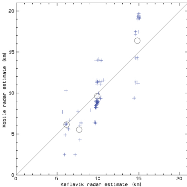
Figure 6. Comparison of synchronous plume-top altitude estimates by the two radars. The circles show mean values of clusters for the Keflavík radar elevation angles (see Table 3).
