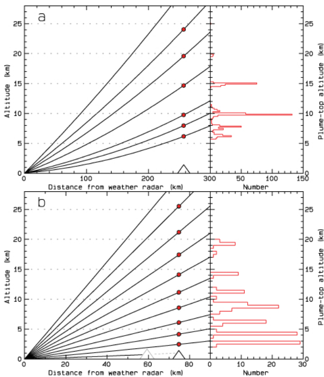
Figure 2. Left: a range-height diagram of the altitude (km a.s.l.) as a function of distance from the weather radars (km), for the lowest elevation angles of the scanning strategy during the eruption. The location of Grímsvötn is marked with a black triangle. Right: a histogram of the plume-top altitudes (km a.s.l.) observed by the radars. (a) Range-height diagram and histogram of altitude estimates from the C-band Keflavík weather radar. The seven lowest elevation angles ( 0.5\text{--}6.0^\circ ) are shown. (b) Range-height diagram and histogram of altitude estimates from the X-band mobile weather radar located close to Kirkjubæjarklaustur. The eleven lowest elevation angles ( 0.5\text{--}23.8^\circ ) are shown. Note that the lowest elevation angle is blocked by the Þórðarhryna mountain, marked by a gray triangle.
