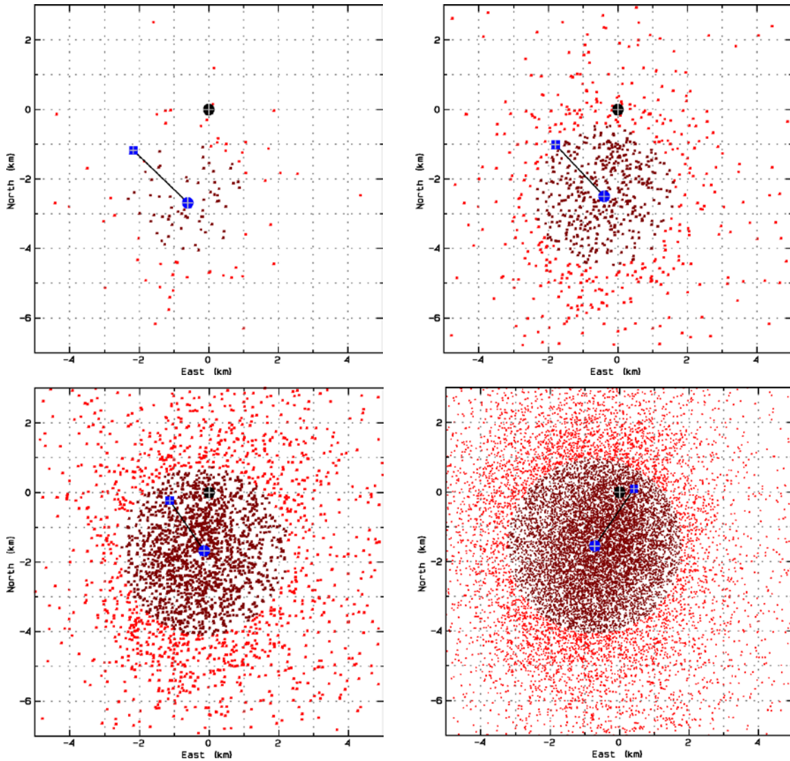
Figure 5. A map view, North (km) vs. East (km), of Grímsvötn 2011 lightning for the first 30 min (123 lightning), 1 hour (888), 3 hours (3340) and 24 hours (16041). The actual eruption site is marked with a black circle with a gray cross at the origin (0,0), the median location of the lightning with a blue circle. Individual lightning are red and brown dots, the closest half of the dots to the median are brown. A backtraced wind correction of the median is shown by the line and blue square. The wind at the 500 hPa level of a weather model was used and this wind backtraced for 500 s.
