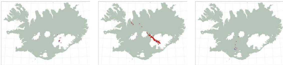
Figure 3. Located lightning prior to the installation of the Keflavík ATD out-station. (a) The Icelandic LLP locations during Grímsvötn 1998. (b) The ATD locations during Grímsvötn 1998. (c) the LLP locations during Hekla 2000. A blue circle is at the vent location.
