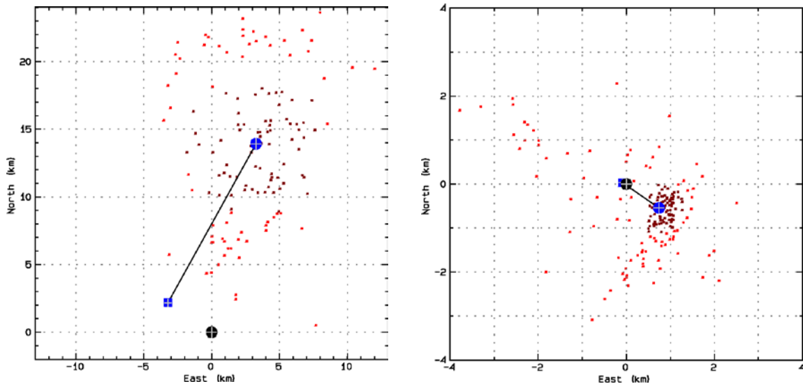
Figure 7. A map view, North (km), vs. East (km) of (a) Grímsvötn 2004 lightning for the first 24 hours (142 lightning) and (b) Eyjafjallajökull 2010 for one day with the highest lightning frequency, 16 May (196 lightning). Note that a different time constant was applied for Eyjafjallajökull wind correction. The labels are the same as in Figure 5.
