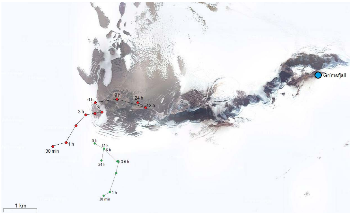
Figure 6. Aerial view of Grímsvötn after the 2011 eruption, with the eruption crater visible in the SW-corner of the caldera (close to the 9 h red dot) about 6 km W of the Grímsfjall station. The eruption site estimates are shown for the first 30 min, 1, 2, 3, 4, 5, 6, 9, 12 and 24 hours of the eruption. The green dots indicate the median lightning locations and the red dots the locations after a simple wind correction with a time constant of 500 s. Four hours into the eruption (at 22:00 UTC) the wind corrected estimates are all within 1 km of the actual eruption crater.
